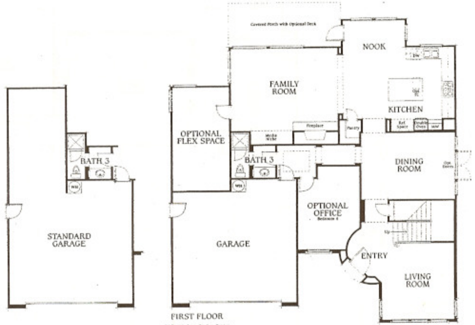
FIRST FLOOR Walls, Windows, Doors, Egress, Doors & Drills 1/4" on Center.
